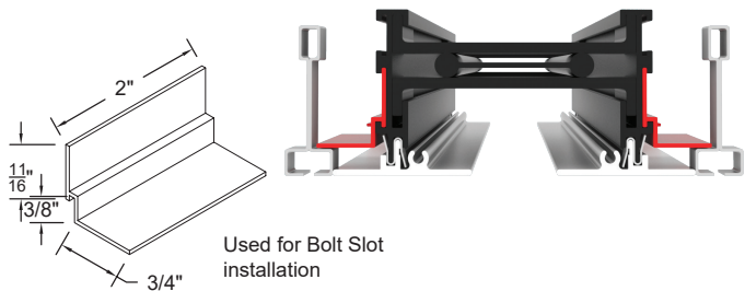
F23 Mounting Hardware
